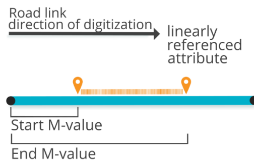
Linearly referenced line attribute data for road links (e.g. speed limit).
